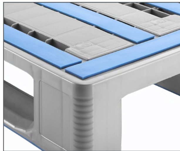
The unique Palgrip ® anti-slip panels are made from high quality HDPE and are permanently part of the deck...
